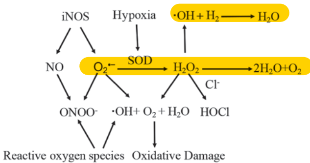
Figure 2. Impact of key oxidants of H 2 in cancer: ·OH and ONOO · are highly reactive to damaged cells, while ·OH, NO · and H 2 O 2 have physiological roles as signaling molecules. H 2 , hydrogen; OH, hydroxyl radicals; ONOO · , peroxynitrite; ·O 2 ·- , superoxide anion; NO, nitric oxide; H 2 O 2 , H 2 peroxide; Cl - , chloride; H 2 O, water; iNOS, inducible nitric oxide synthase; SOD, superoxide dismutase.
